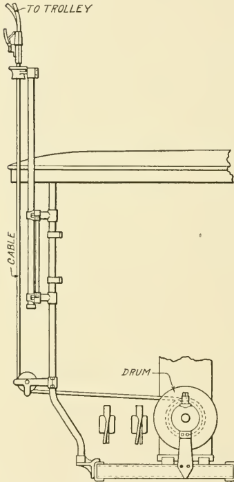
Fig. 8. Details of Trolley Cable Winding Drum
